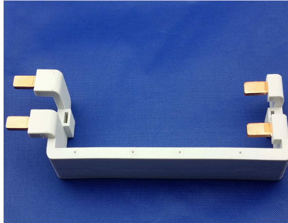
Inlay copper part, high voltage tested
