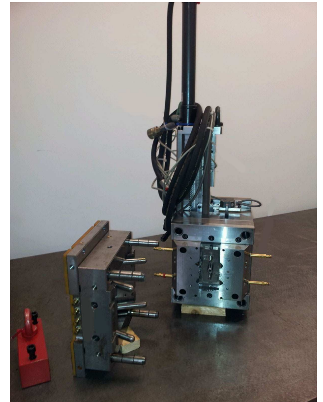
Mould with gear box and sliders
